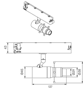
ZTA.35.MAINS TRACK.FRAME - FIXED BEAM
