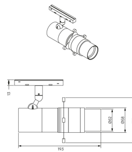
ZTA.50.LV.TRACK FRAMER - FIXED BEAM
