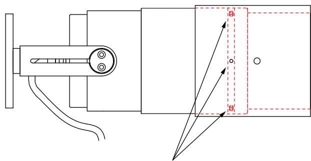
Remove the 3 x M3 fixings to remove the snoot.
